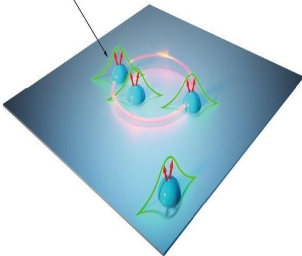
Majorana and e/4 quasiparticles
